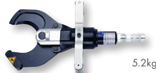
85mm Cutting Head ACSR/Steel Part No. SDK85C
