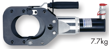
105mm Armoured Cutting Head Part No. SDG105C
